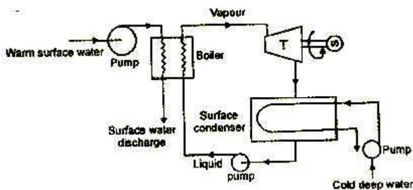
Figure: OTEC – closed cycle
