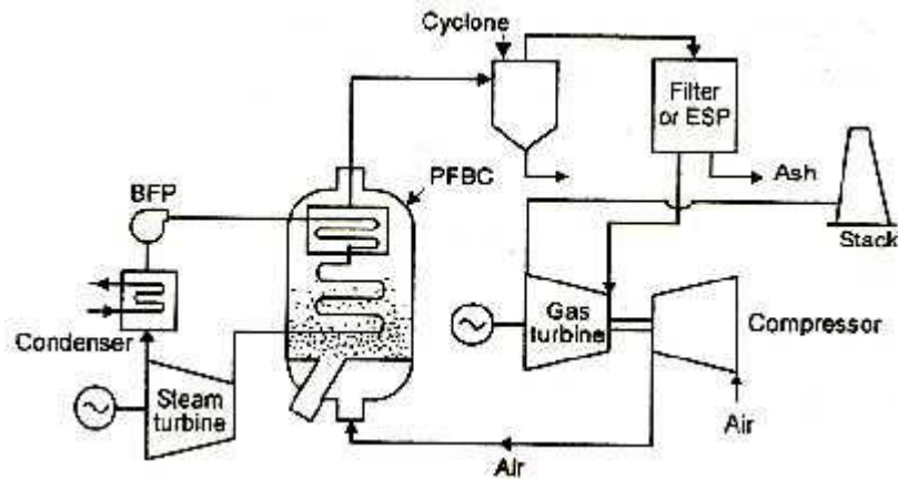
Figure: PFBC turbocharged arrangement
