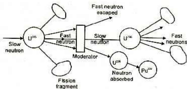
Figure: Nuclear fission.
