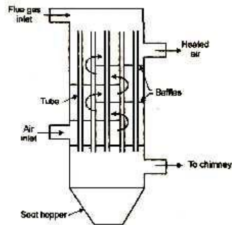
Figure: Air pre-heater
